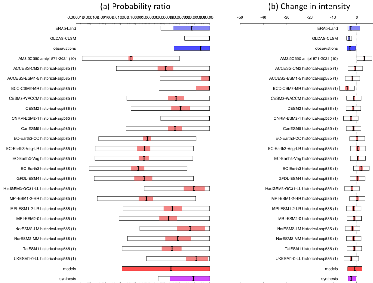
Fig. 10: Synthesis of (a) probability ratios and (b) intensity changes (%) when comparing the return period and magnitudes of the 2022 JJA root zone soil moisture for the NHET region in the current climate and a 1.2°C cooler climate.
